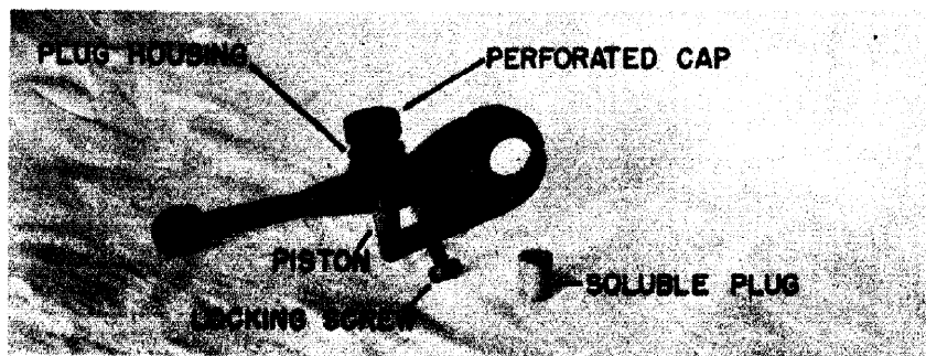
Fig. 32. Automatic Clamp
